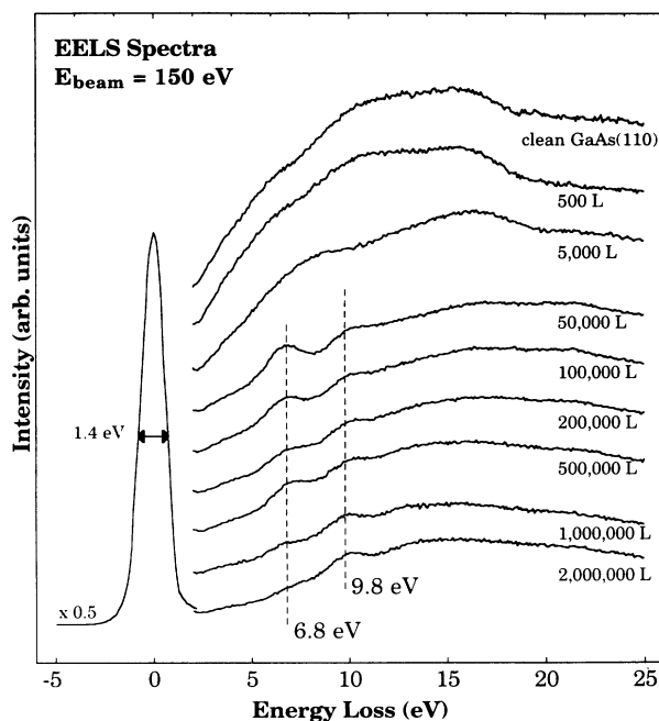
FIG. 5. EELS spectra collected from a GaAs(110) wafer, and from the same wafer after increasing exposures to XeF 2 . The combined resolution of the electron beam and detector is 1.4 eV. Two loss features at 6.8 and 9.8 eV are apparent in the spectra collected from the fluorinated samples, and correspond to transitions from the GaF 3 VBM to the GaAs CBM and GaF 3 CBM, respectively.
