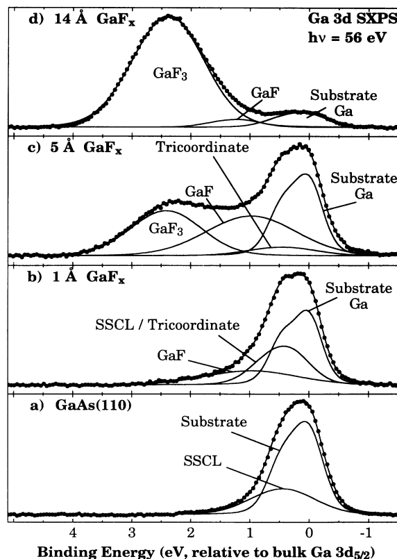
FIG. 3. High-resolution SXPS spectra of the Ga 3d core level, collected from GaAs(110) before and after exposure to XeF 2 , are shown along with the results of numerical fits to the data. The raw data after background subtraction are shown as solid circles. The solid lines show the individual and the sum of the components of the fit. (a) shows the core level from the clean surface, and (b)–(d) contain core levels from fluorinated surfaces.
