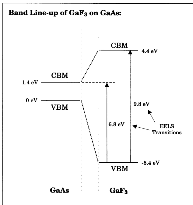
FIG. 6. The band lineup, based on the SXPS and EELS measurements, of GaF 3 films grown on GaAs wafers via exposure to XeF 2 . The energies of the band edges are given with respect to the GaAs VBM. The electronic transitions responsible for the EELS features are indicated.
