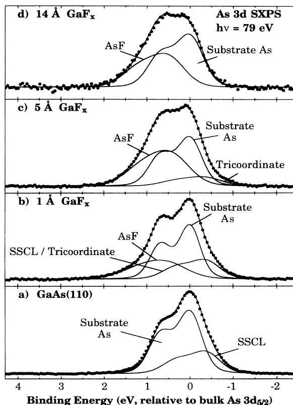
FIG. 4. High-resolution SXPS spectra of the As 3d core level, collected from GaAs(110) before and after exposure to XeF 2 , are shown along with the results of numerical fits to the data. The raw data after background subtraction are shown as solid circles. The solid lines show the individual and the sum of the components of the fit. (a) shows the core level from the clean surface, and (b)–(d) contain core levels from fluorinated surfaces.
